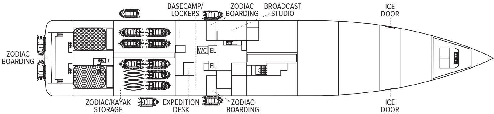
EXPEDITION DECK
